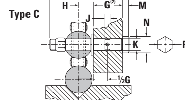
Type C If set screws are used to lock pin they should be at right angles to applied load Cantilever Type Trunnion Pin—Thru-hole
