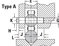
Type A If set screws are used to lock pin they should be at right angles to applied load Straddle Type Trunnion Pin
