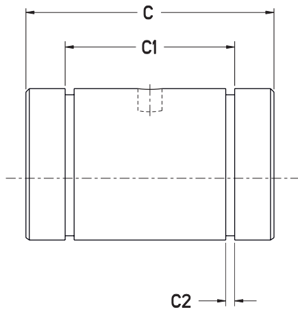
Dimensions [mm]
