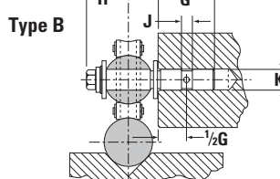
Type B If set screws are used to lock pin they should be at right angles to applied load Cantilever Type Trunnion Pin—Blind Hole
